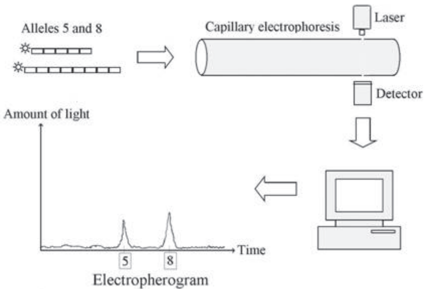
Figure 3. Sketch of an electropherogram for two D16S539 alleles. One allele has five repeats of the sequence GATA; the other has eight. Each GATA repeat is depicted as a small rectangle. Although only one copy of each allele (with a fluorescent molecule, or “tag” attached) is shown here, PCR generates a great many copies from the DNA sample with these alleles at the D16S539 locus. These copies are drawn through the capillary tube, and the tags glow as the STR fragments move through the laser beam. An electronic camera measures the colored light from the tags. Finally, a computer processes the signal from the camera to produce the electropherogram. Source: David H. Kaye, The Double Helix and the Law of Evidence 189, fig. 9.1 (2010).
